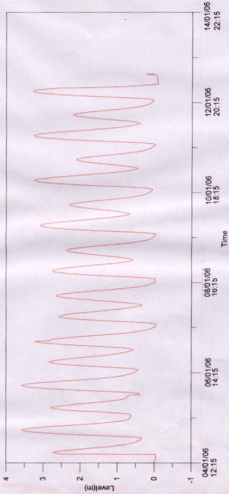
Figure 4.2.1: Tide collected at Kotdi Creek during 4 to 12 January 2006
